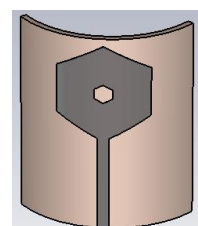
Fig. 9 Conformal configuration of hexagonal patch Antenna with hexagonal slot
