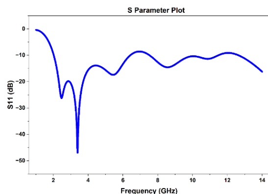
Fig. 2 Simulated reflection coefficient ( S_{11} ) of the Hexagonal microstrip patch antenna
