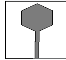
Fig. 1 The geometry of the Hexagonal microstrip patch antenna
