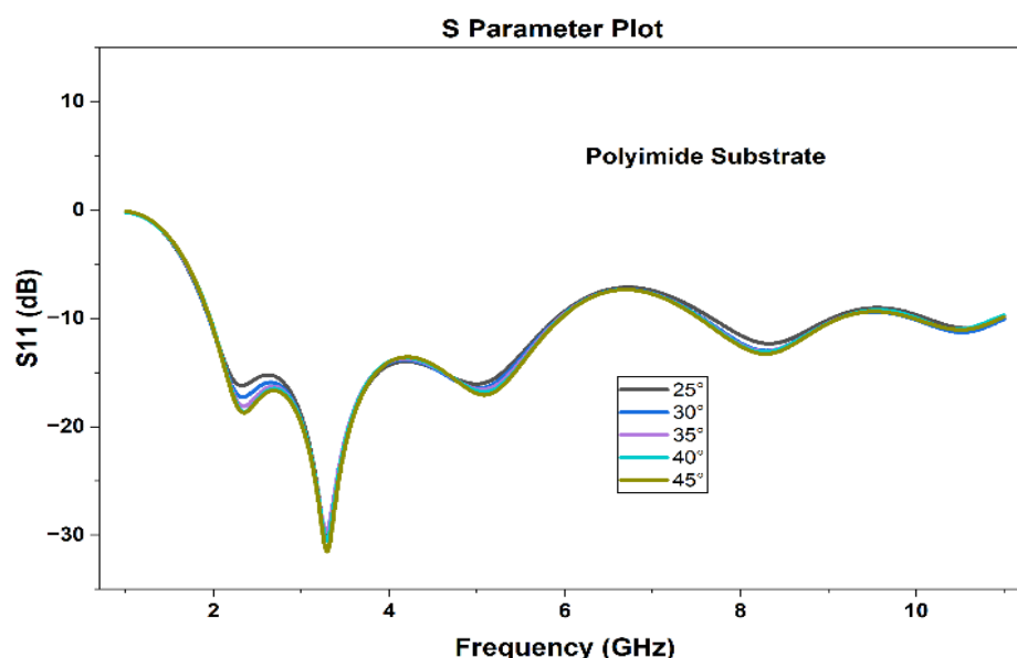
Fig. 12. Reflection coefficient comparison of conformal (25° - 45° bent) configurations for the hexagonal patch Antenna with hexagonal slot with Polyimide substrate
