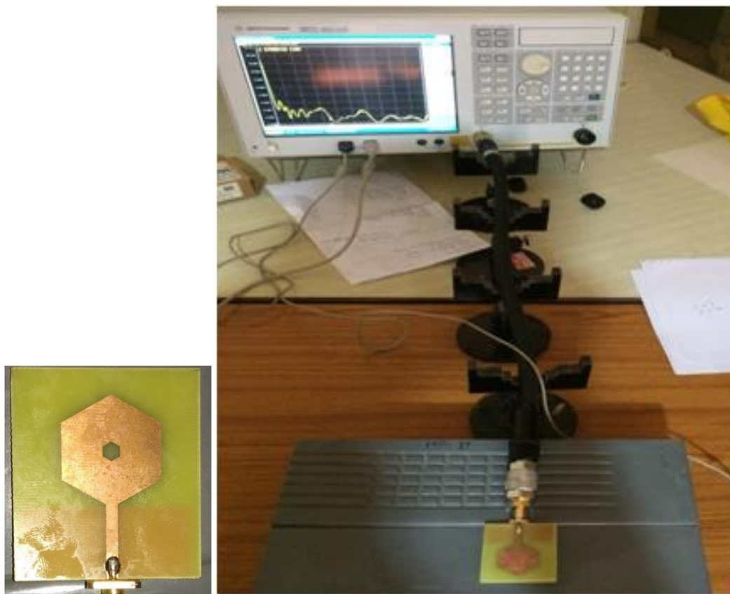
Fig.13 Fabricated Structure and Experimental Setup of the Antenna
