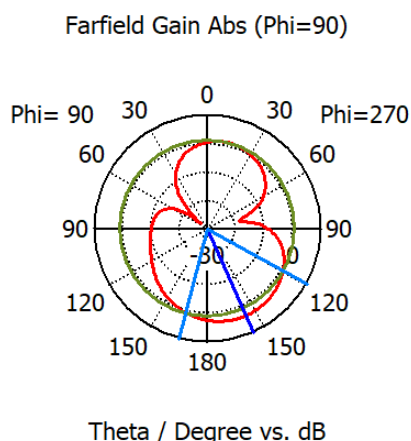
Fig. 3 Far-field radiation pattern ( \Phi = 90^\circ plane) of the hexagonal patch Antenna at the resonant frequency
