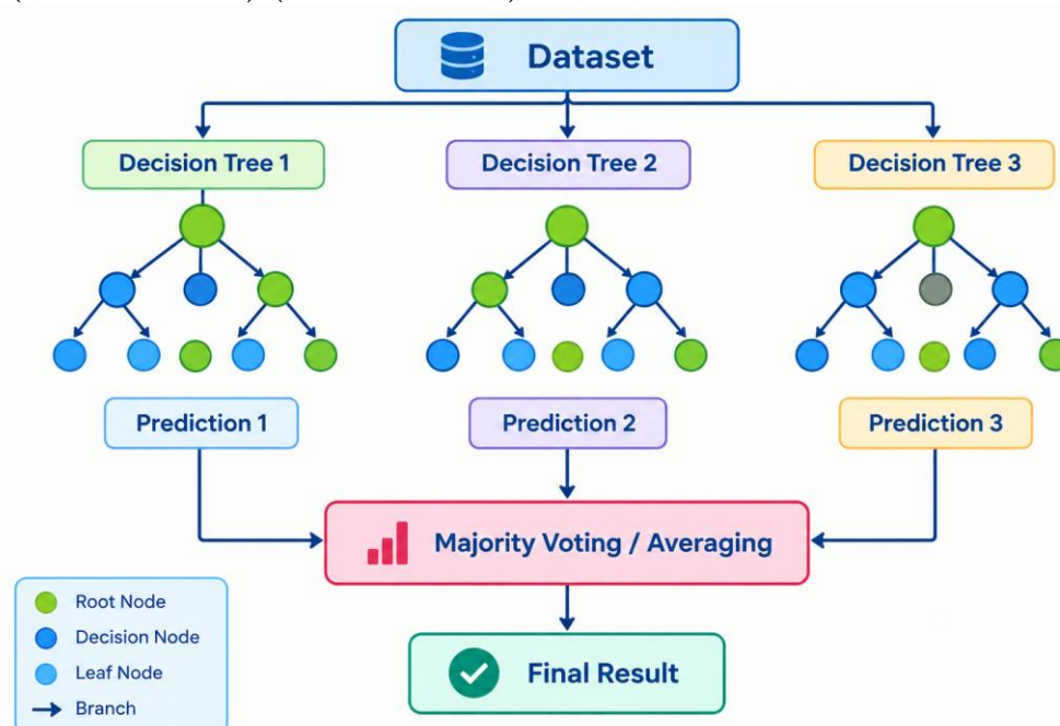
Figure. 1 Random Forest
