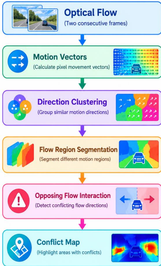
Figure. 2 Process of motion conflict detection to detect interacting flows in pedestrians.
