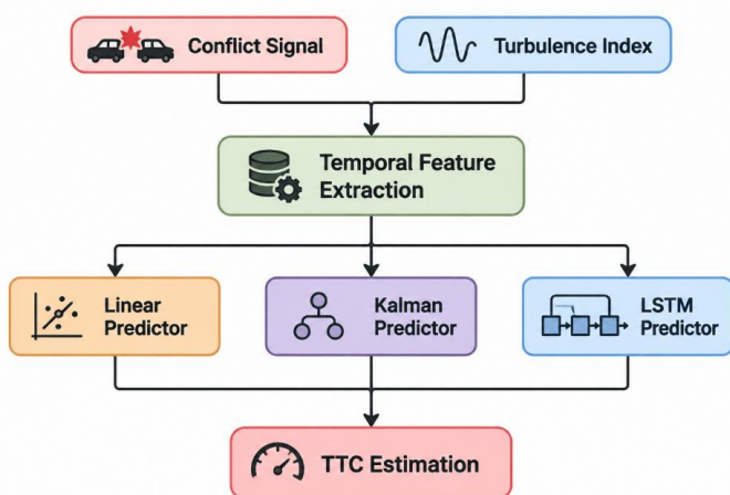
Figure. 3 Temporal prediction models that are based on estimating time-to-congestion.
