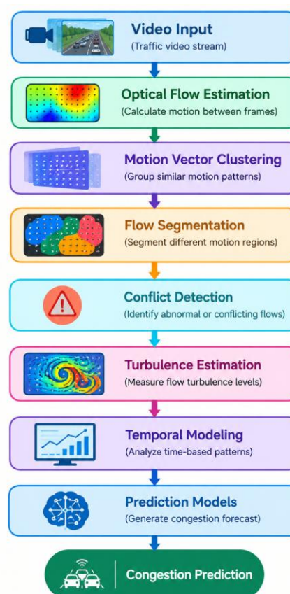
Figure. 1 Design of the suggested turbulence-conscience crowd congestion prediction architecture.
