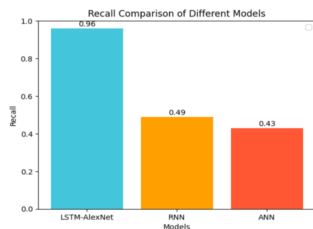
Fig.4 Recall Comparison of Models
