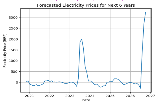
Fig.6 Forecasted Electricity Prices for Next 6 Years
