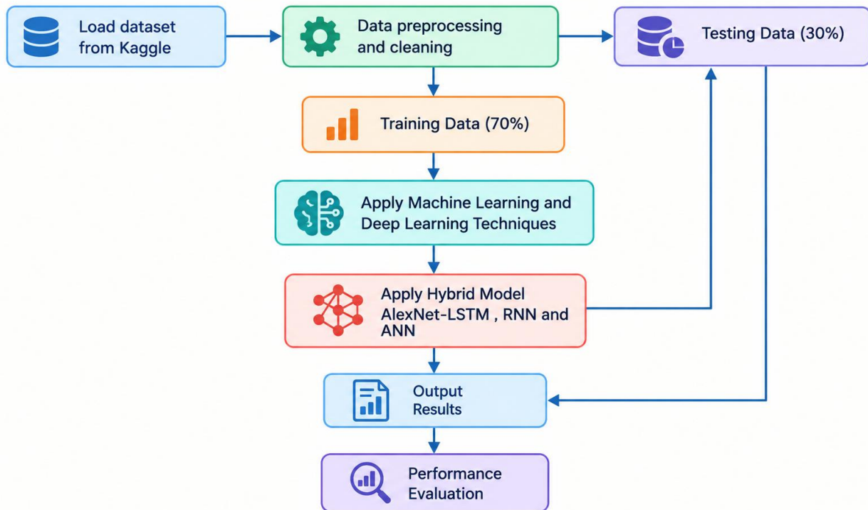
Fig.1 Architecture of Electricity Price Prediction Model
