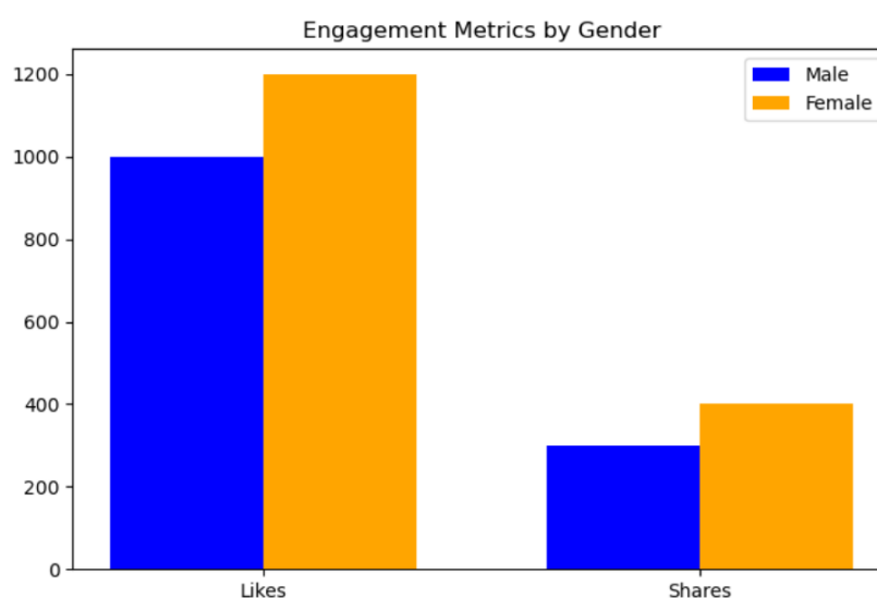
Fig.7 Engagement Metrics by Gender.
