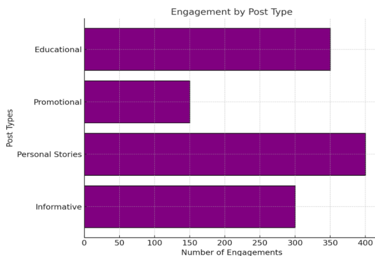
Fig 10. Number of Engagement by Post Type.
