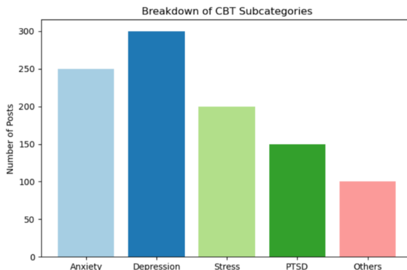
Fig 6. Breakdown of CBT Subcategories.
