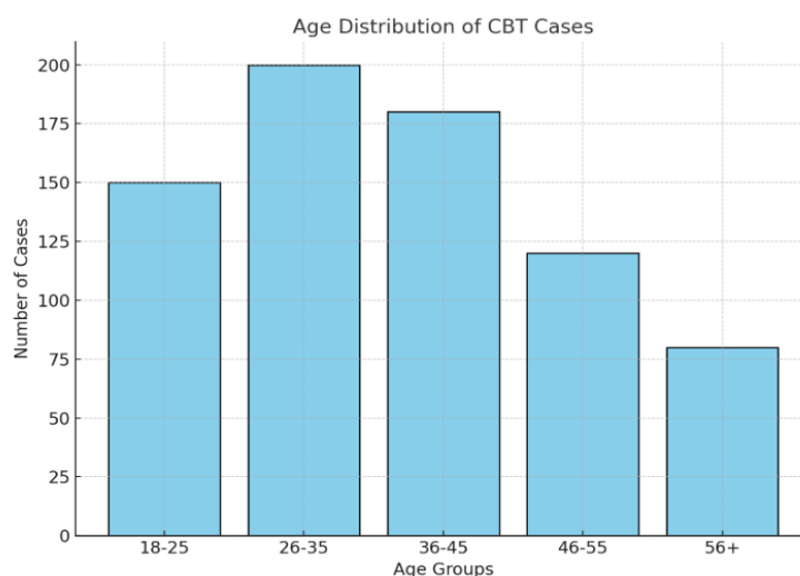
Fig 8. Age Distribution of CBT Cases.
