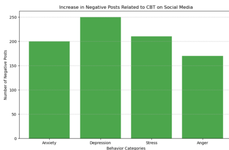
Fig 3. Increase in Negative Posts Related to CBT on Social Media.
