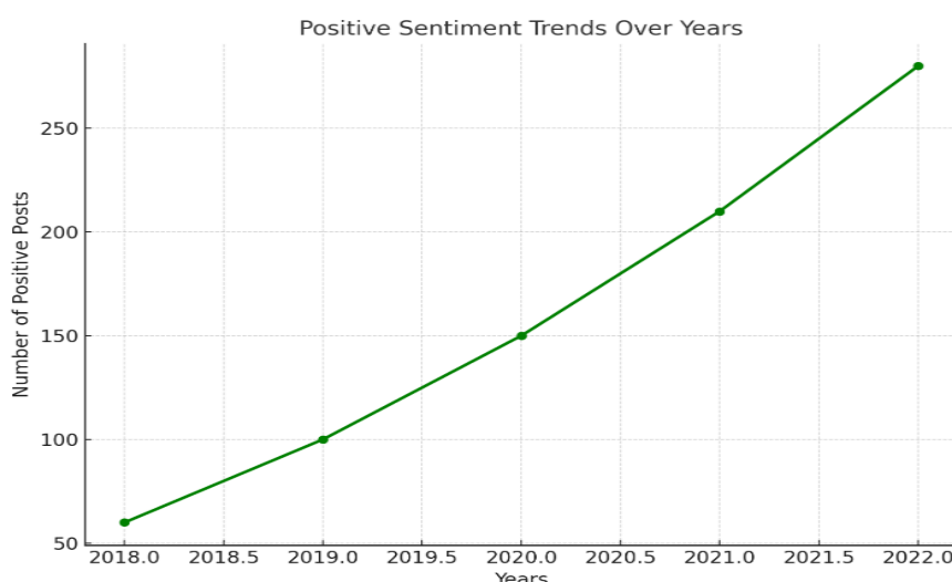
Fig.9 Positive Sentiment Trends Over years.
