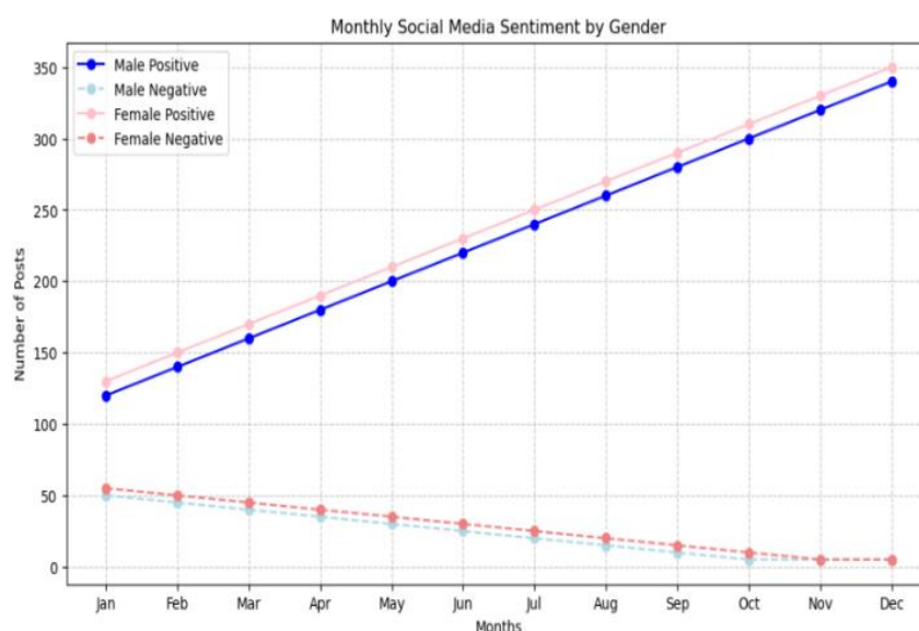
Fig 4. Monthly Social Media Sentiment by Gender.
