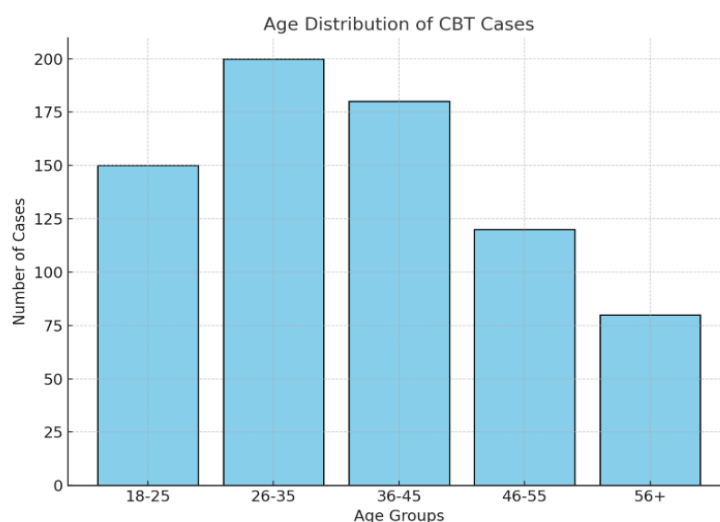
Fig.5 Age Distribution of CBT Cases.
