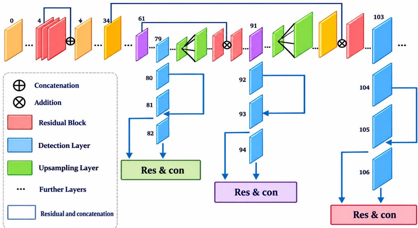
Figure. 3 Proposed model (CAR connection)
