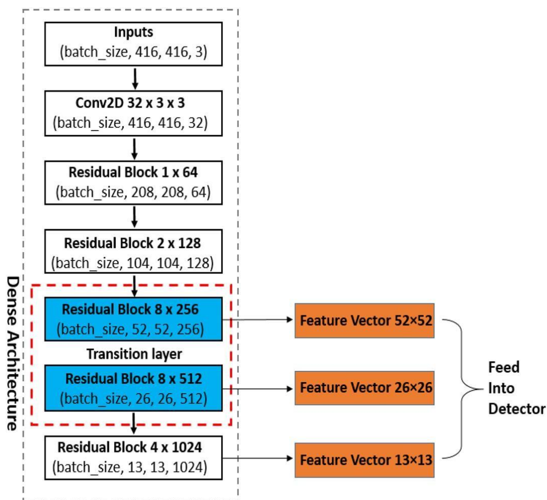
Figure. 2 Yolo-V3 model
