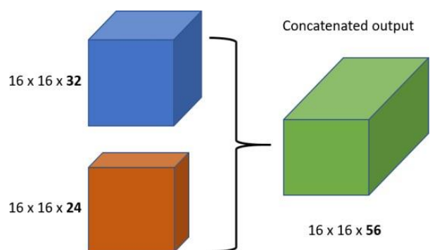
Figure. 5 Concatenation connection
