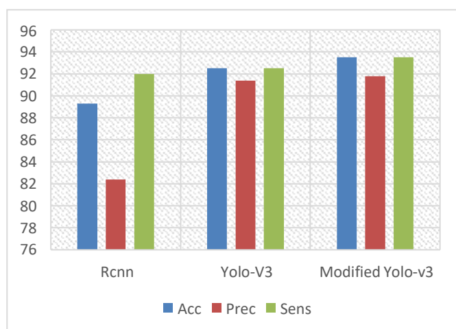
Figure. 10 Detection With Normalisation
