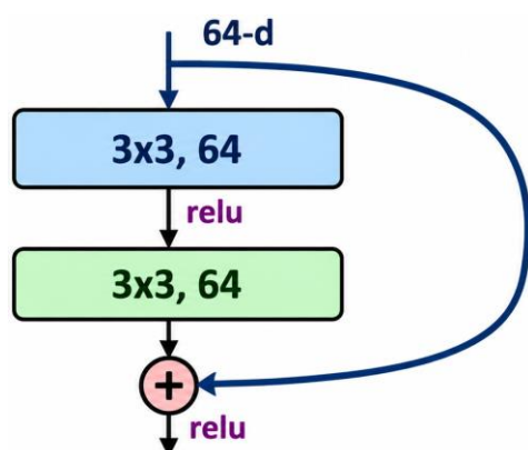
Figure. 4 2-layer Skip connection
