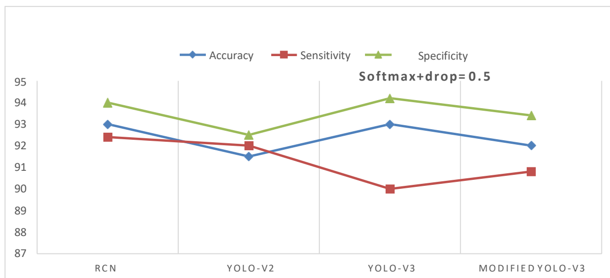
Figure. 12 In case of Dropout 0.5
