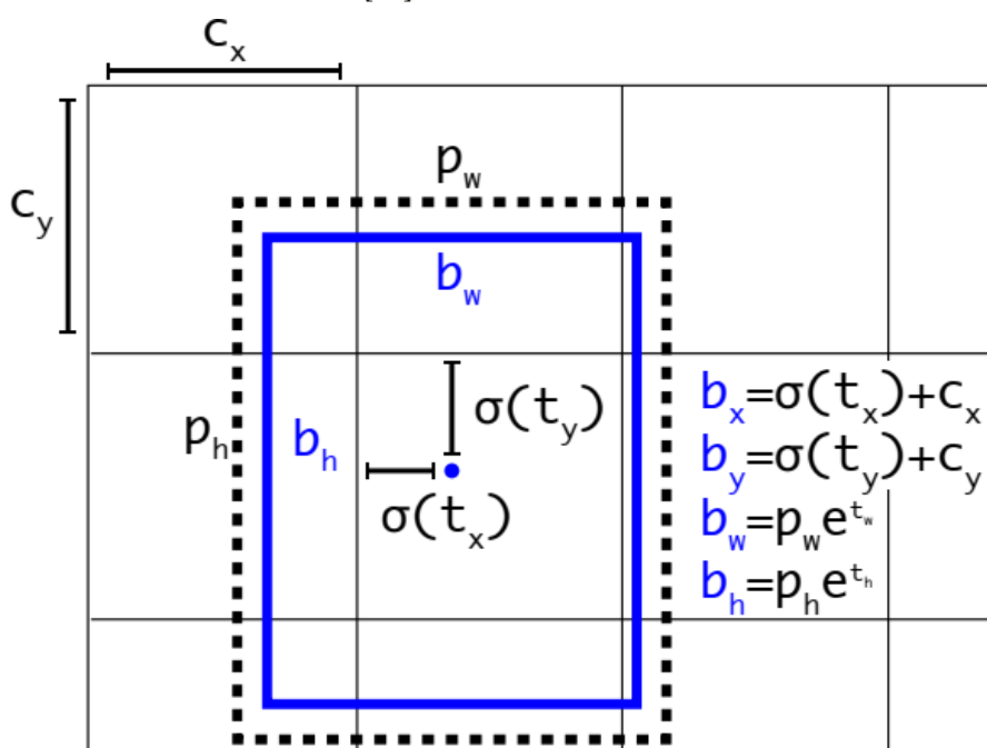
Figure. 1 Bounding boxes with location and dimension priors
