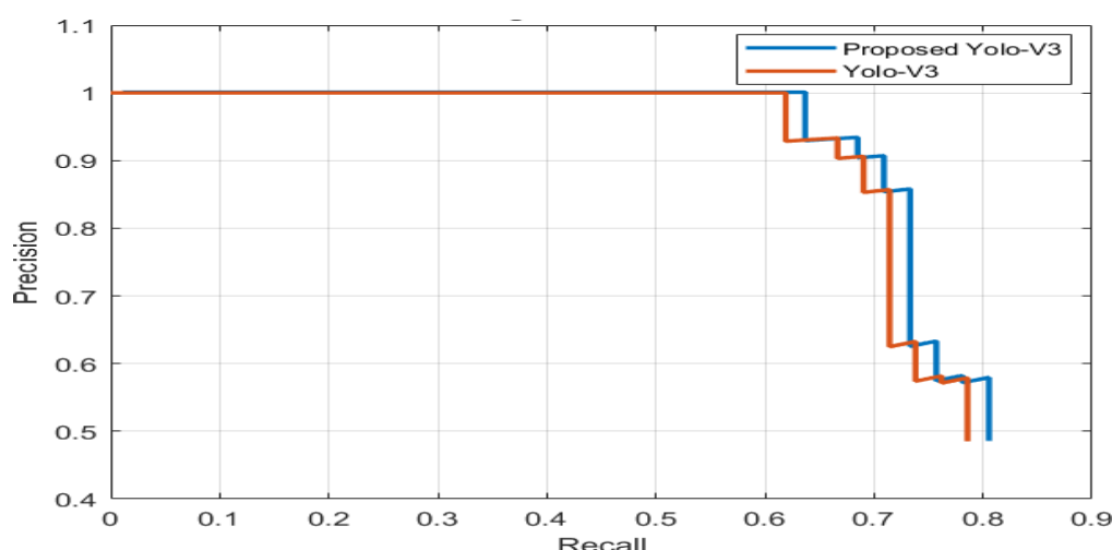
Figure. 7 Map curve for the system
