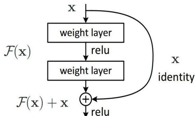
Figure. 4 Skip connections
