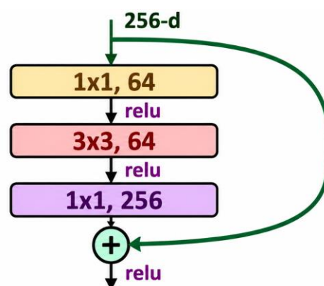
Figure. 5 3-layer Skip connection
