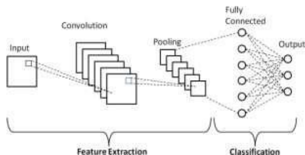
Figure. 2 CNN architecture
