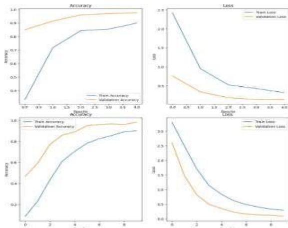
Figure. 4 CNN Accuracy and Loss
