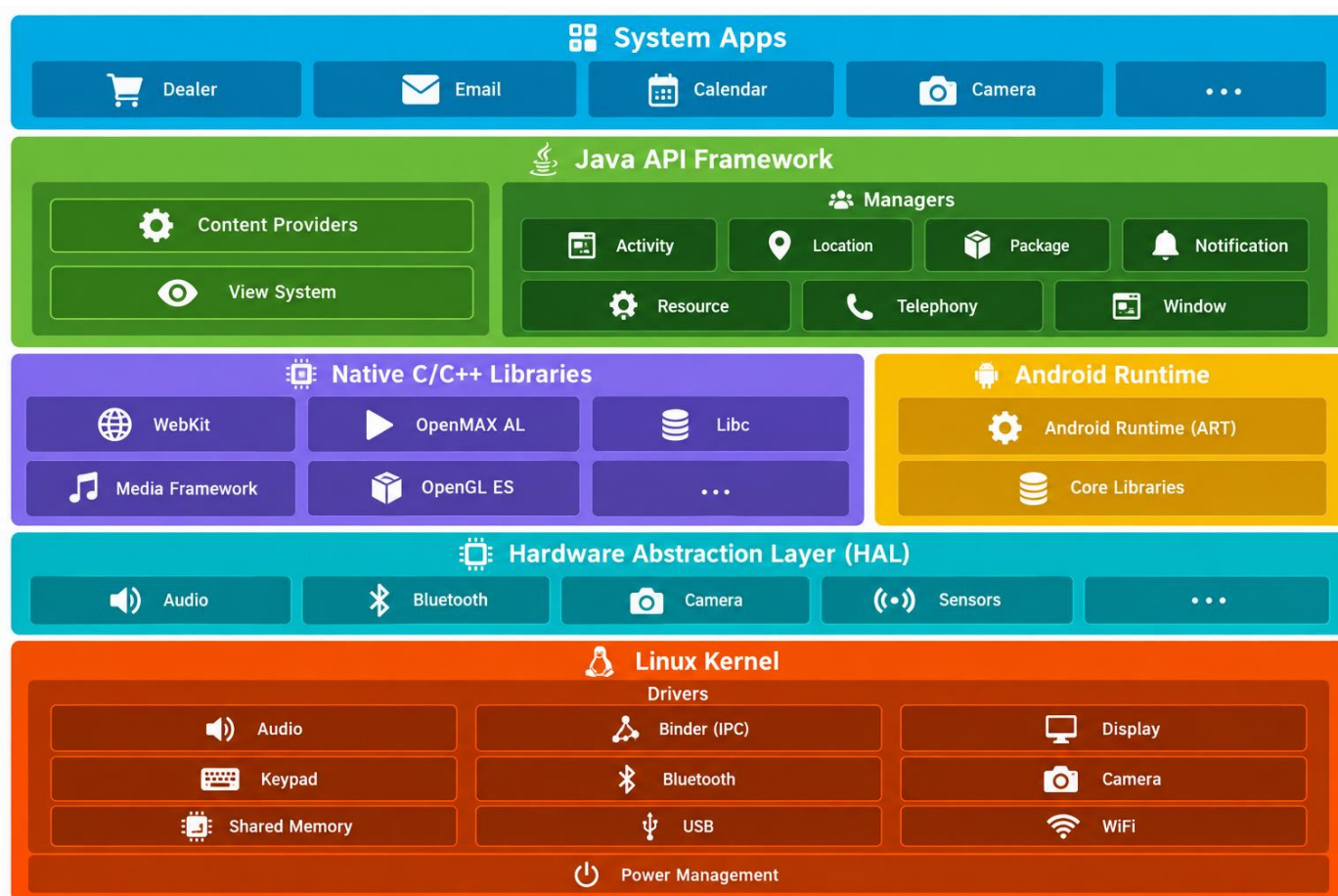
Figure. 1 Android Architecture
