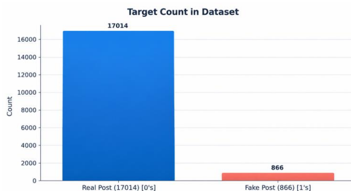
Figure. 2 Dataset plot
