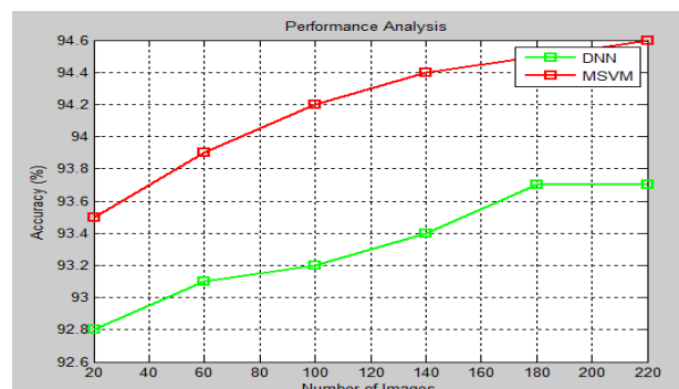
Figure. 7 Showing accuracy performance of both classifiers
