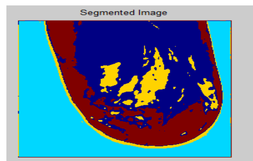
Figure. 3 Segmented image
