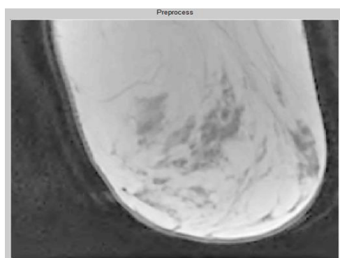
Figure.2 Pre-processed image
