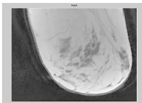
Figure.1 Input image
