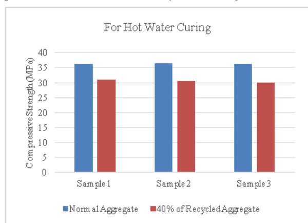
Figure. 1 Shows the Compressive Strength Comparison between Concrete with Normal Aggregate and Concrete with 40% Recycled Aggregate using Hot Water Curing
