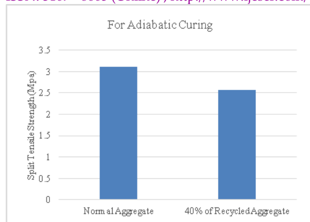
Figure. 6 Shows the Split Tensile Strength Comparison between Concrete with Normal Aggregate and Concrete with 40% Recycled Aggregate using Adiabatic Curing
