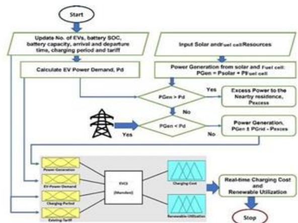
Figure. 5 Proposed energy management system for EVCS
