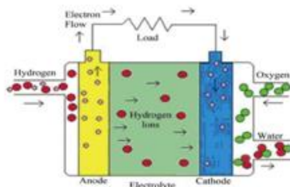
Figure. 3 PEM Cell
