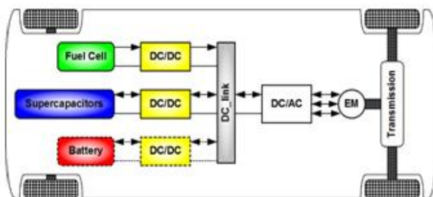
Figure.1 Electric vehicle power train
