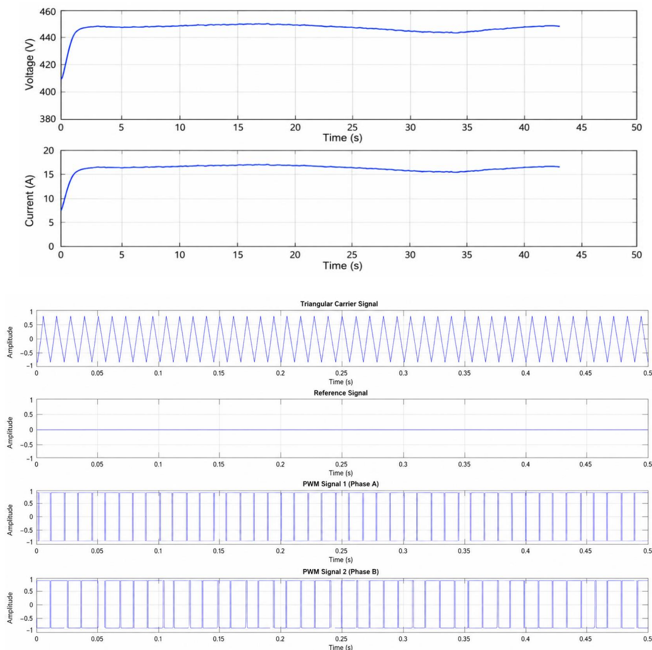
Figure. 5 Rectifier Output and PWM Carrier and reference signal
