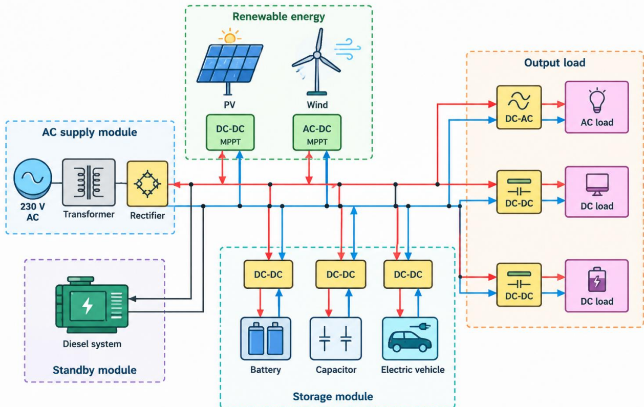
Figure. 1 DC Micro Grid Architecture
