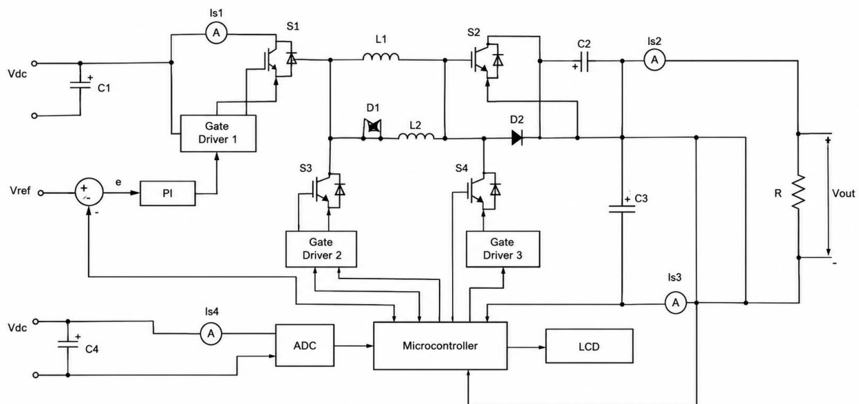
Figure. 4 Subsystem Simulation
