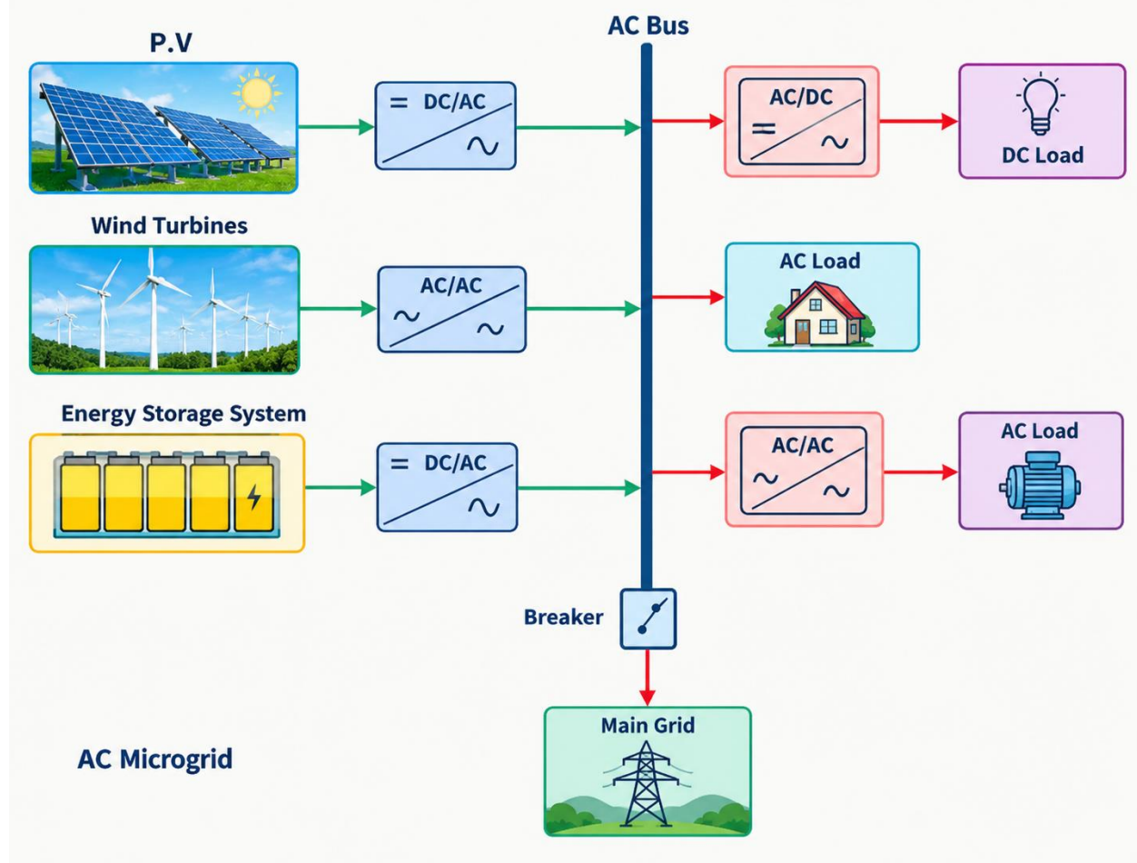
Figure. 2 AC Micro Grid Architecture
