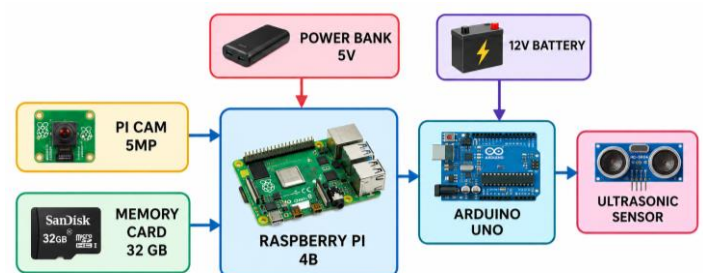
Figure. 3 Identification Model
