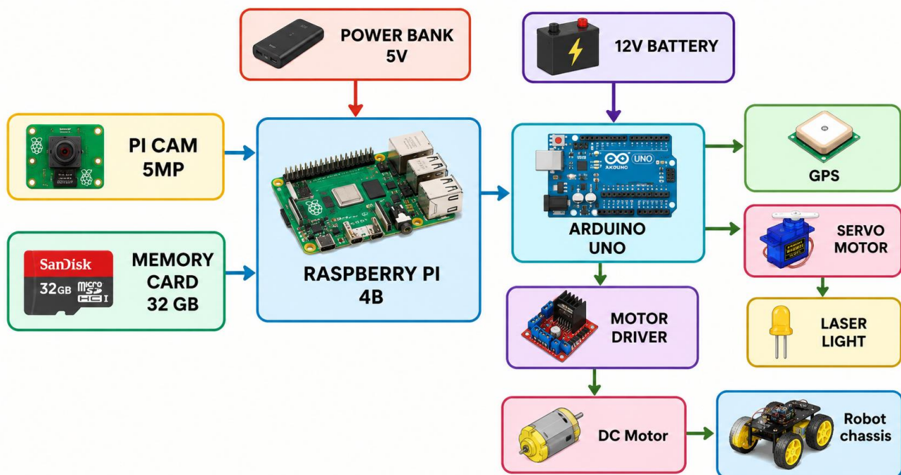
Figure. 4 Neutralization Model
