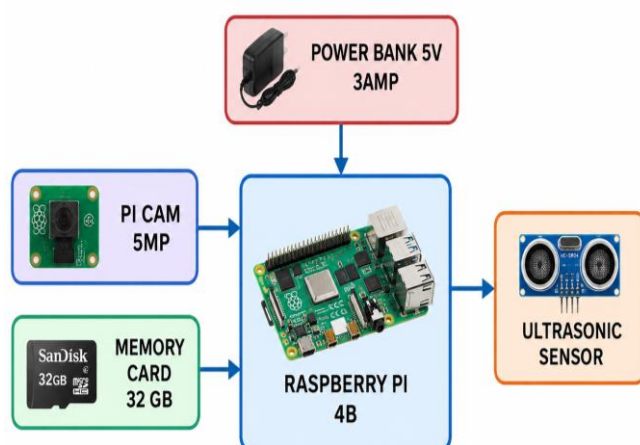
Figure. 2 Detection Model
