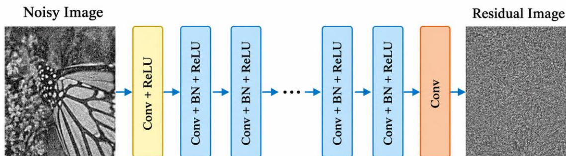
Figure. 1 The architecture of proposed DnCNN network
