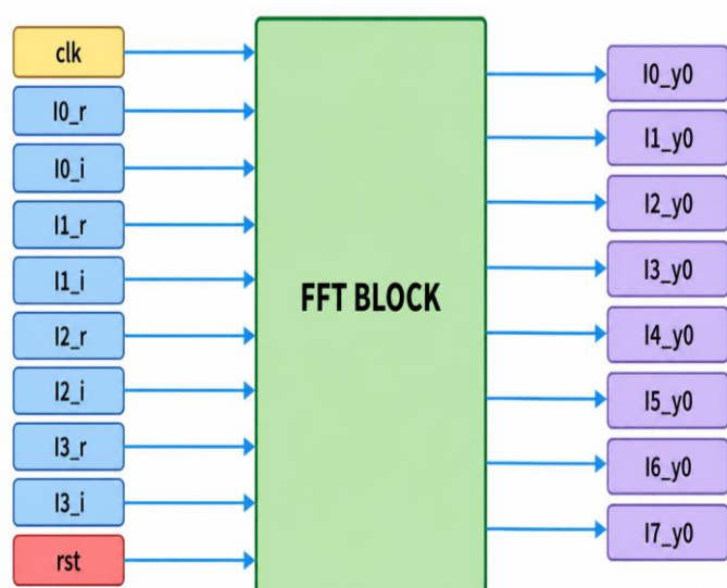
Figure. 4 Input/output block diagram for OTFS 16 bit
