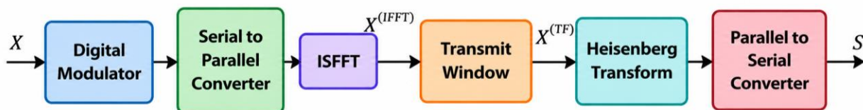
Figure. 1 Block Diagram of Orthogonal Time Frequency Space (OTFS) Modulation
