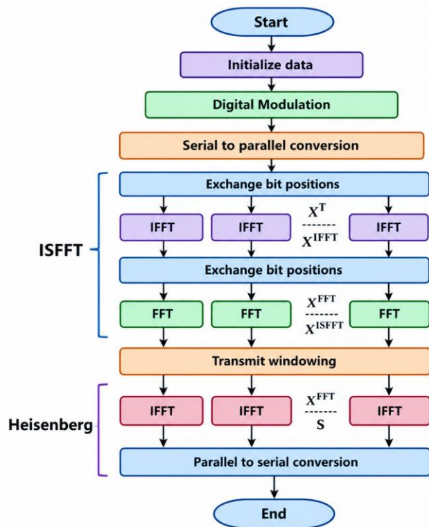
Figure. 2 Hardware architecture of the OTFS transmitter
