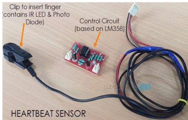
Figure. 4 Heartbeat Sensor Module
