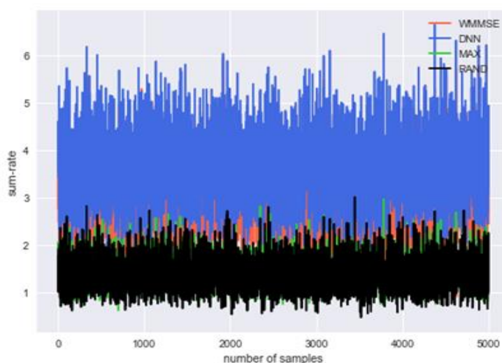
Figure. 3 DNN Sample Performance for k =20 Users
