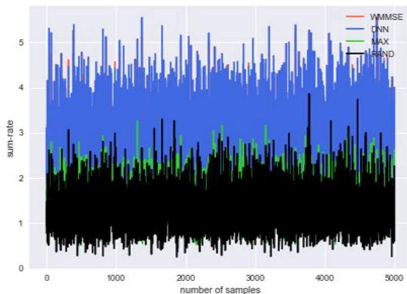
Figure. 1 DNN sample performance for k= 10 users
