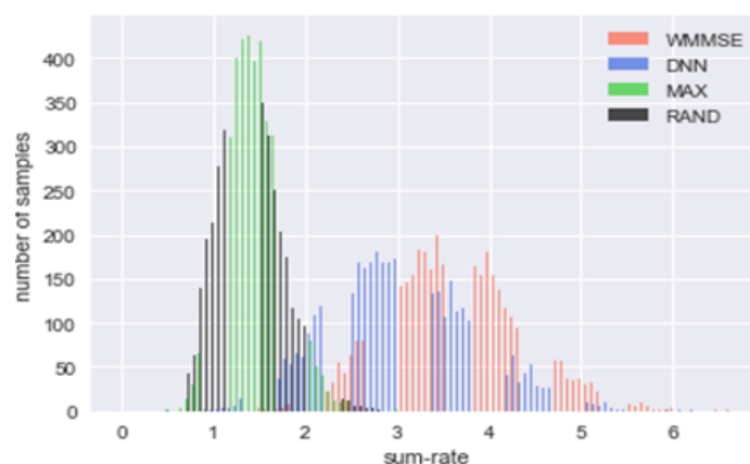
Figure. 4 DNN Sum Rate Distribution for K = 20 Users
