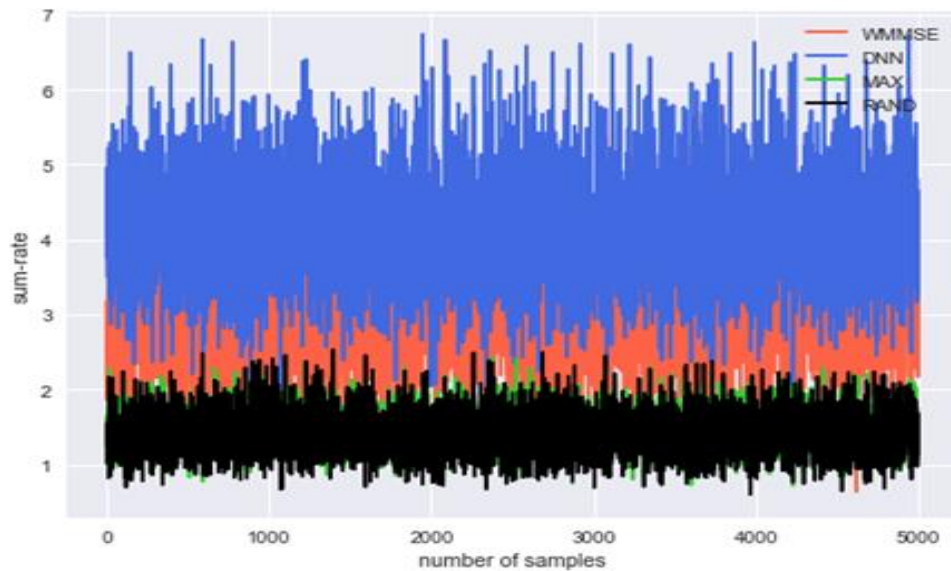
Figure. 5 DNN Sample performance for k = 30 Users
