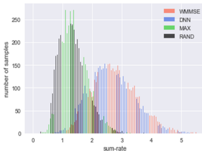
Figure. 2 Sum Rate Distribution for K=10 users
