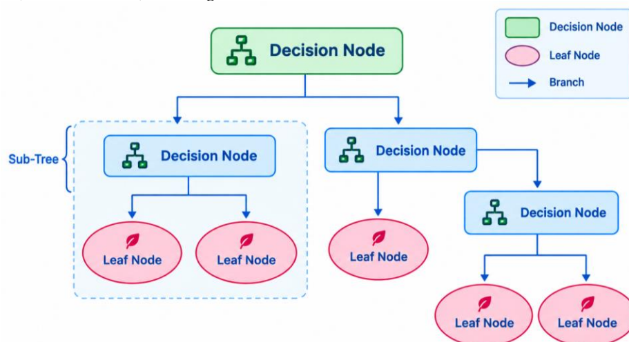
Figure. 1 Working of Decision Tree
