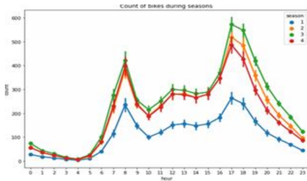
Figure. 8 Graphical Representation (Count of bikes during seasons)
