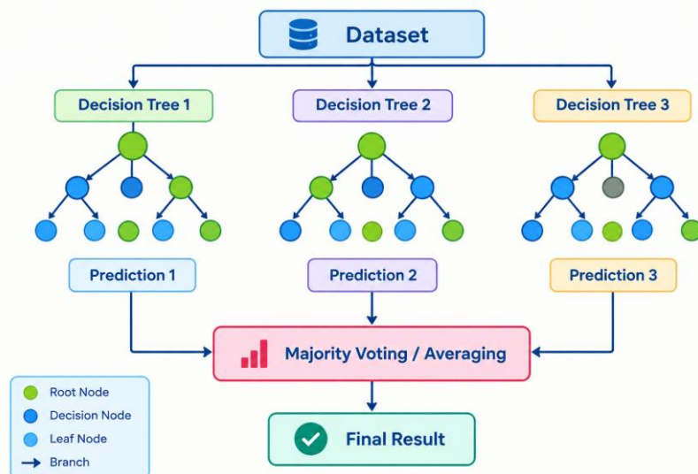
Figure. 2 Working of Random Forest
