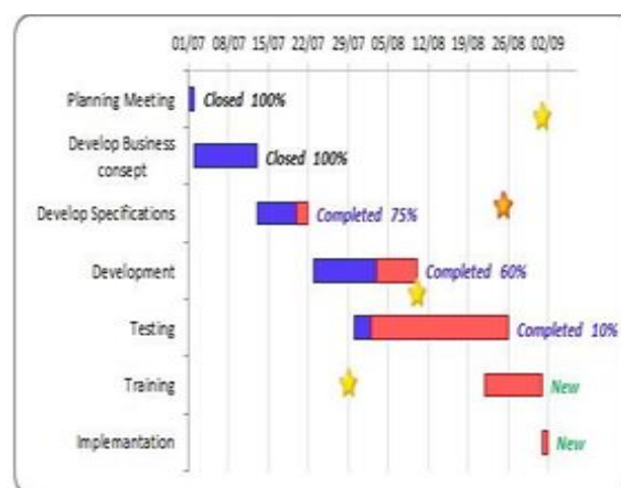
Figure.1 Gantt Char
