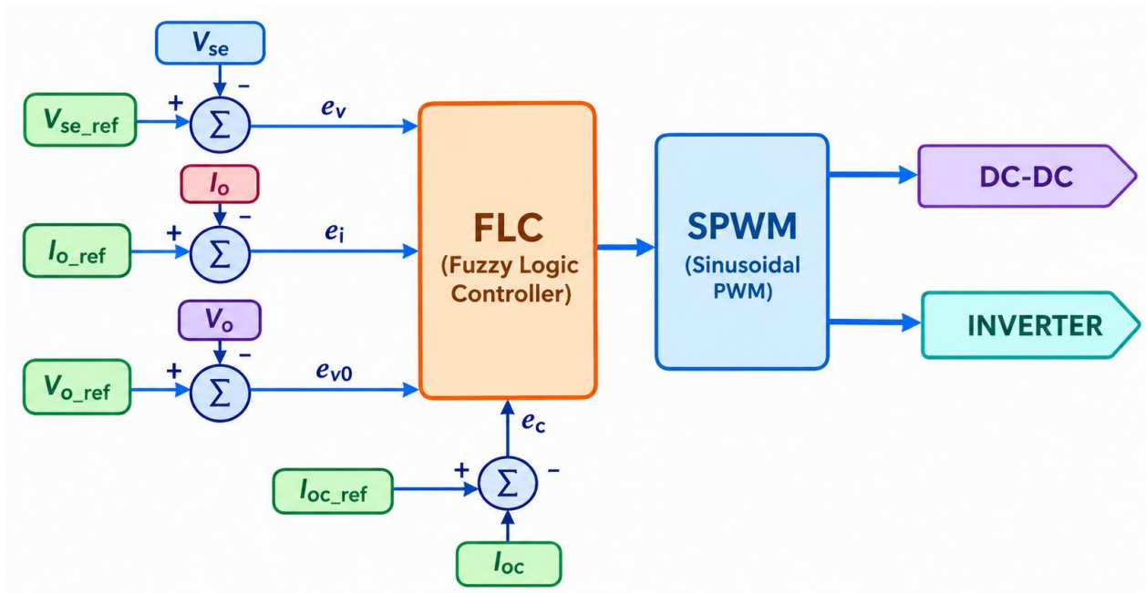
Figure. 4 Proposed V/F Control Block Diagram
