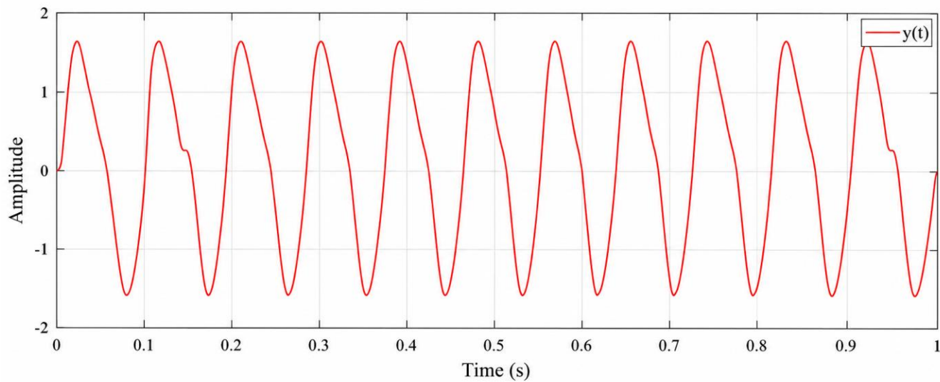
Figure. 13 Battery Current
