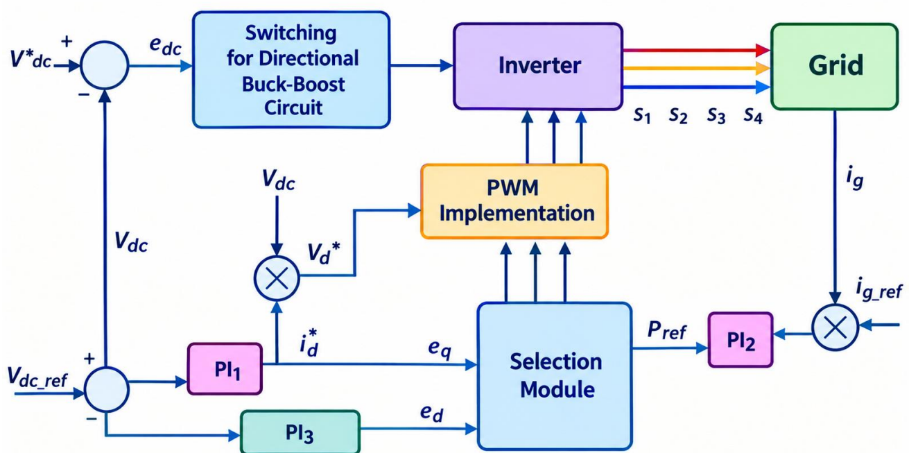
Figure. 2 Proposed Topology
