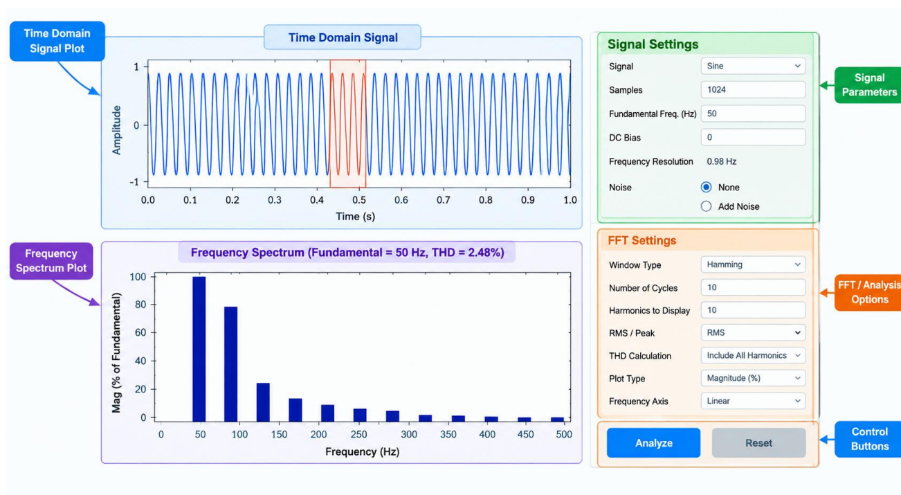
Figure. 10 T.H.D Waveforms (Grid current(A))
