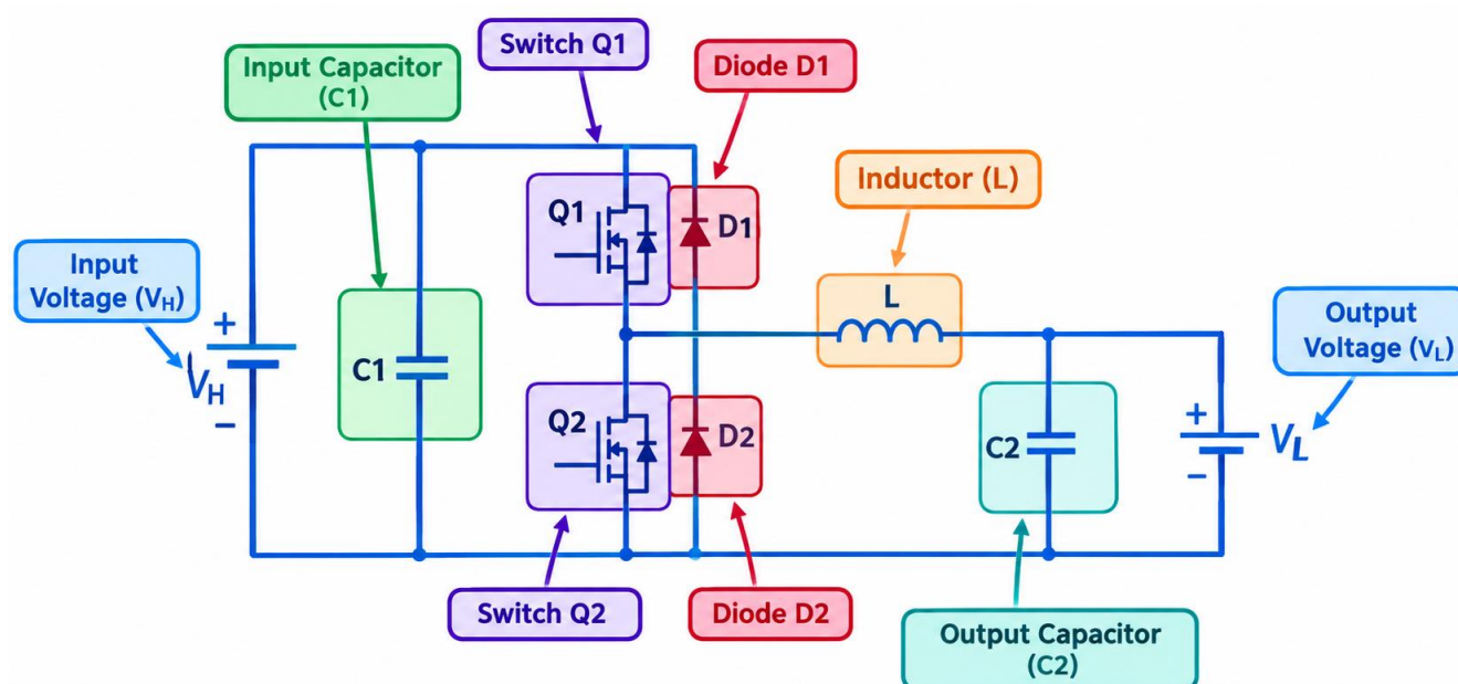
Figure. 1 Bidirectional DC-DC Converter
