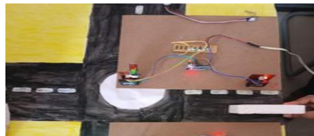
Figure. 3 Ambulance Detection
