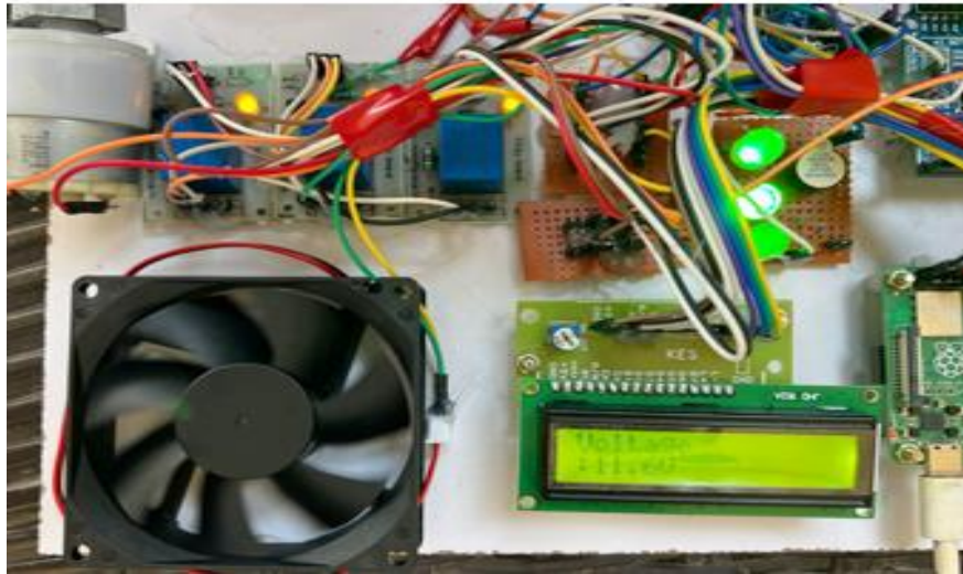
Figure. 11 Real Time Voltage Display
