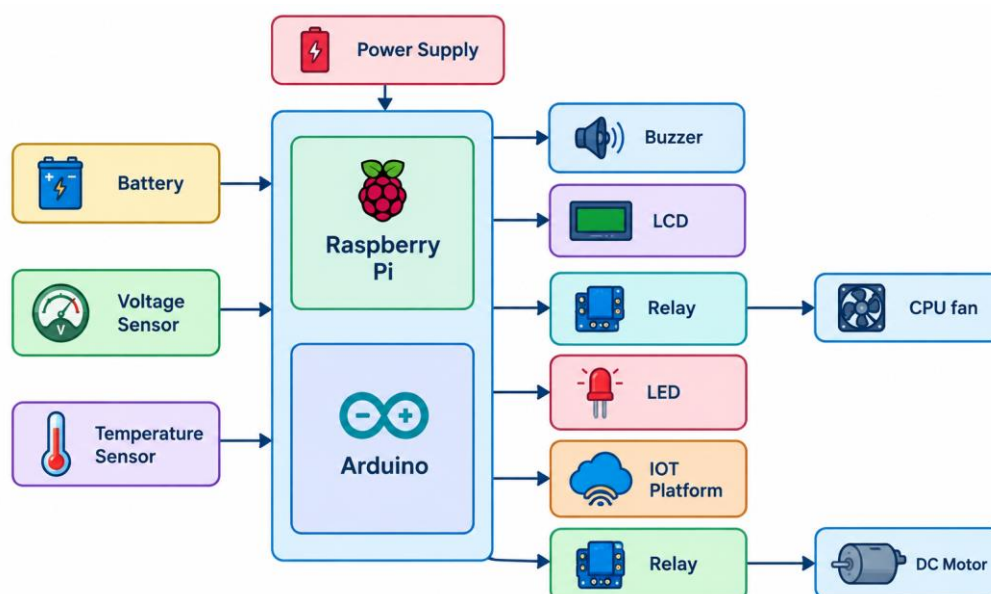
Figure. 9 Block Diagram
