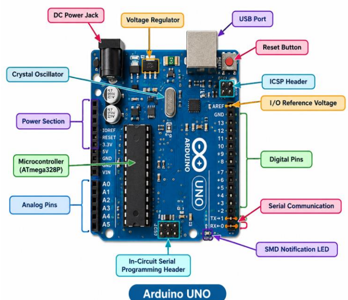
Figure. 2 Ardino UN0
